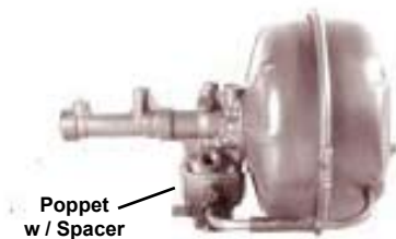
PART NO. 2700385 DOUBLE POPPET W/O BRKT. W/O PLUG
