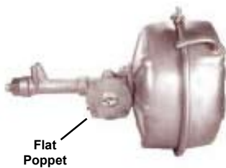
PART NO. 2700383 FLAT POPPET W/O BRKT. WITH PLUG
