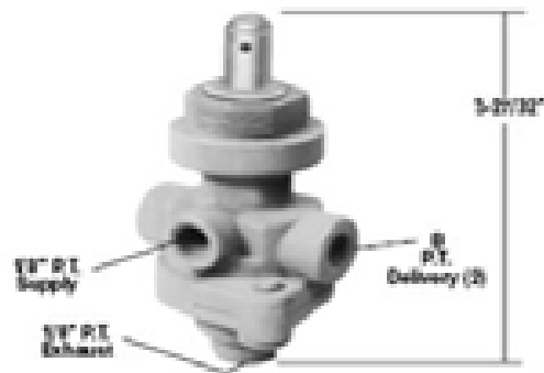
PP-8 PUSH PULL CONTROL PIC #116 - WEIGHT: 1 LB.
