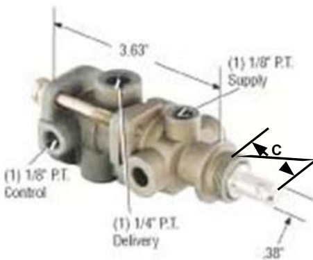
PP-7 TRAILER SUPPLY VALVE PIC #115 - WEIGHT: 1 LB.
